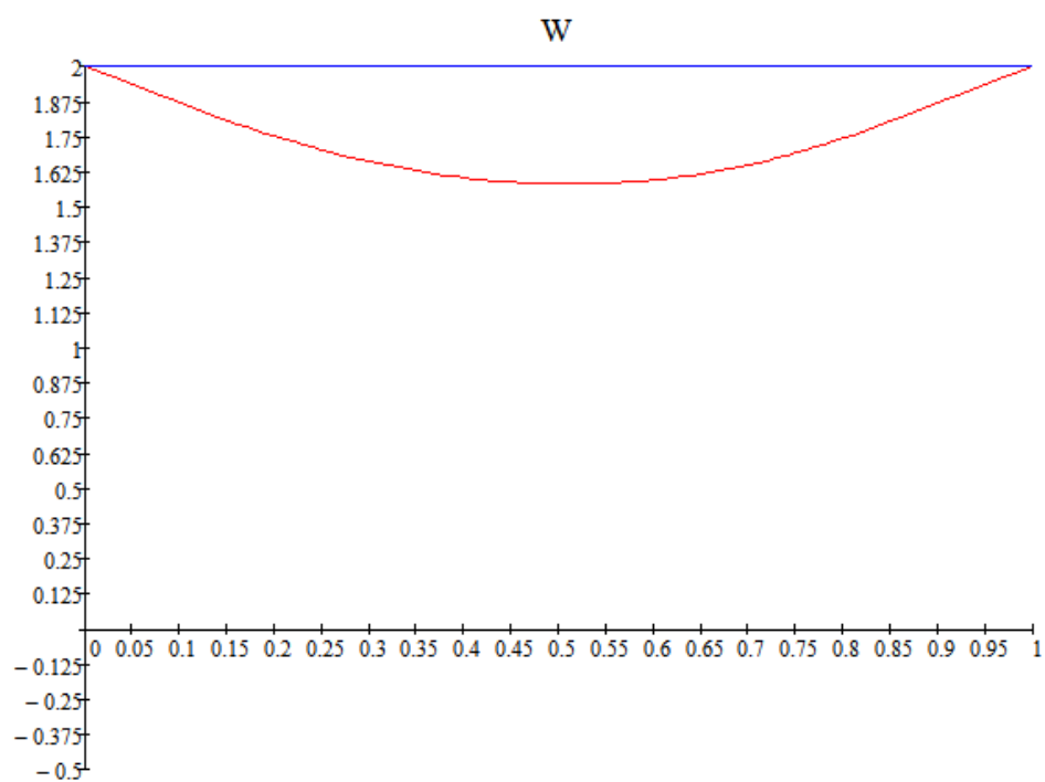
Fig. 3 ( t = 0.1 )
