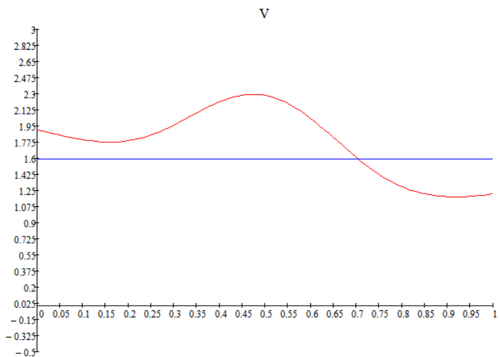
Fig. 4 ( t = 0.1 )
