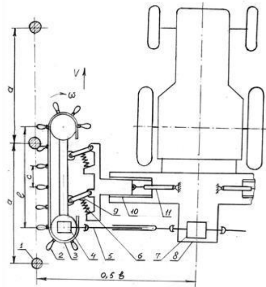
Fig. 1. Scheme of the machine for blowing fruits from the plant with impact oscillations
