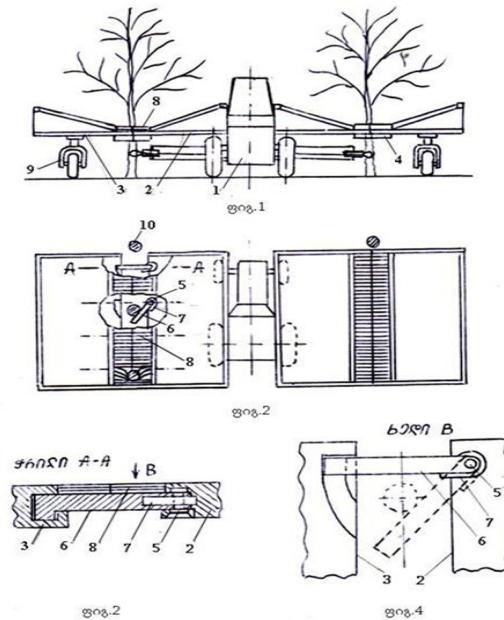
Fig. 2. Device for holding fruits of fruit trees
